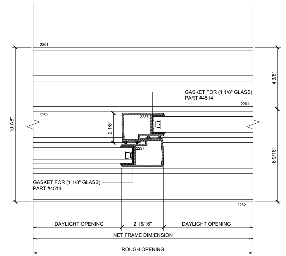
③ VERTICAL MAX SLIDING DOORS (OXXXX-XXXXO) SCALE: 6"=1'-0"
