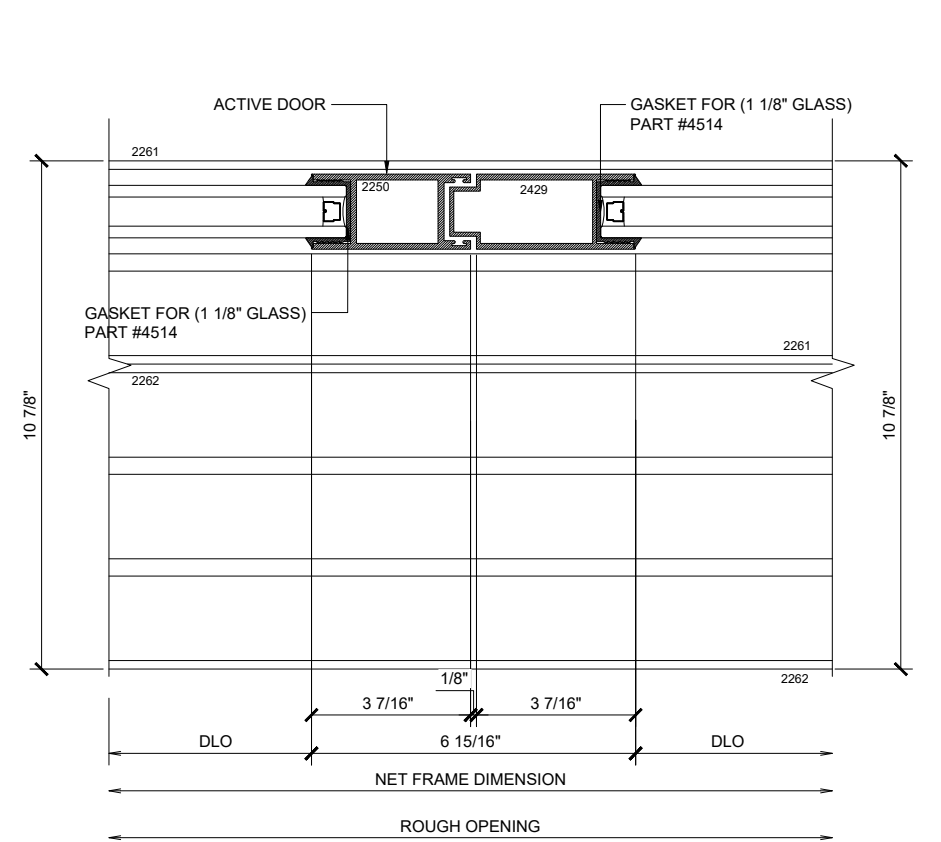
⑥ VERTICAL MAX SLIDING DOORS (OXXXX-XXXXO) SCALE: 6"=1'-0"
